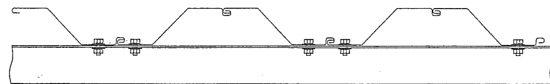
WATER BOLT PLACEMENT (HEAVY "Z" STYLE SHEETS)
