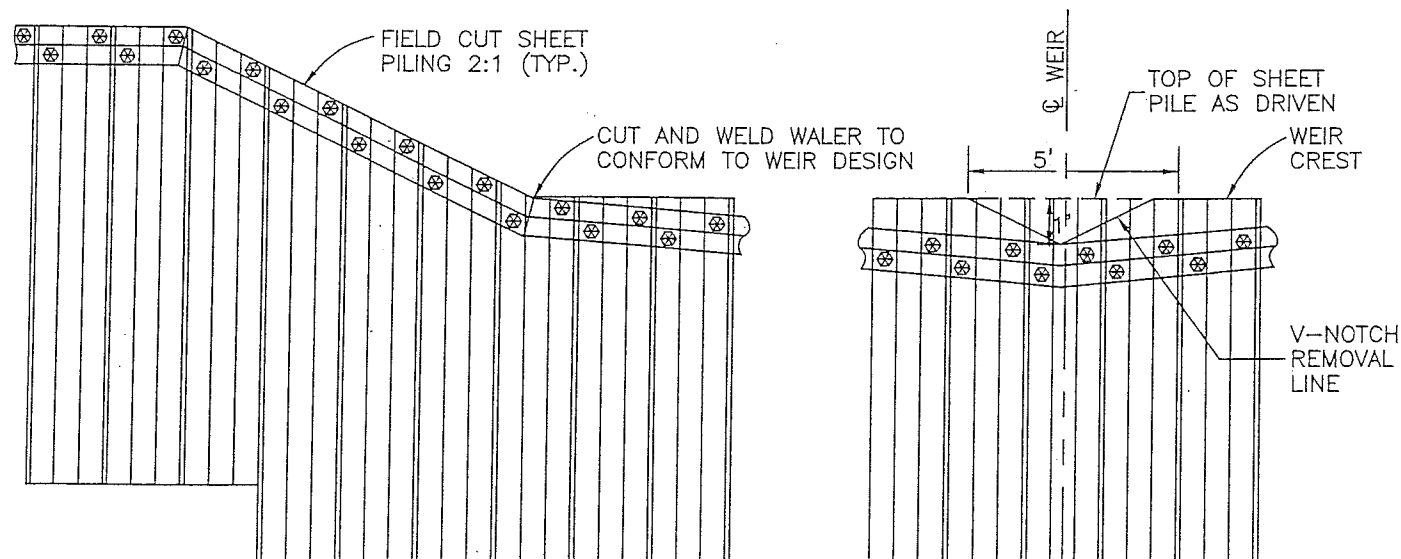
WATER BOLT PLACEMENT (HEAVY "Z" STYLE SHEETS)
