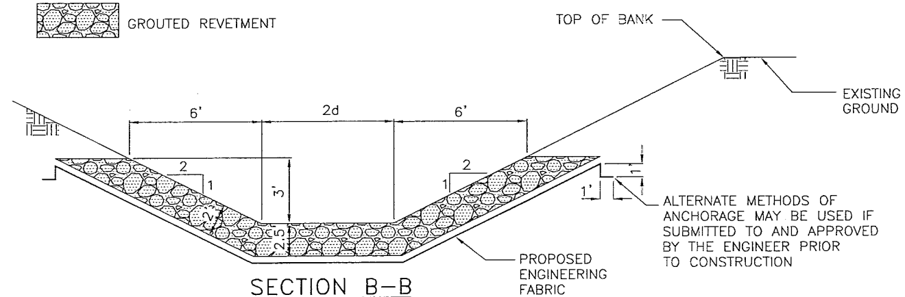
DETAILS OF PREFORMED SCOUR HOLE
