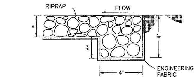
TYPICAL UPSTREAM
