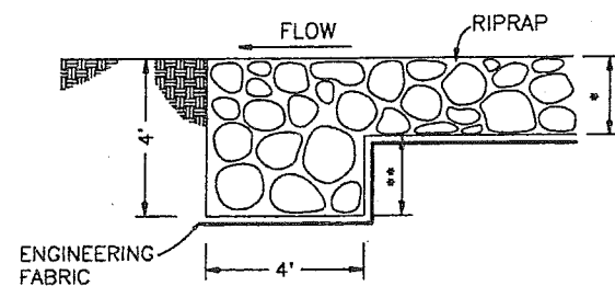
TYPICAL DOWNSTREAM
