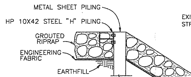
GROUTED RIP-RAP DETAIL
