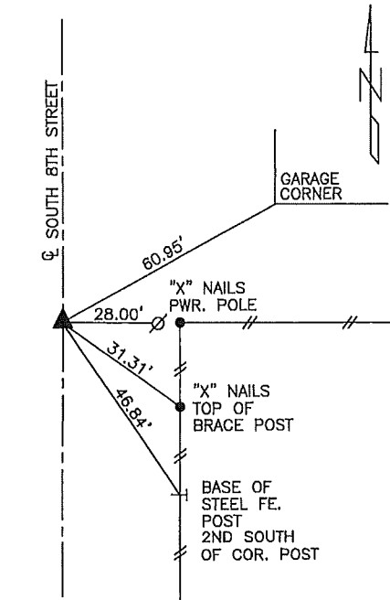
DISTANCES PLUMB CHAINED NE CORNER SE1/4 SE1/4 SECTION 15-83-39
