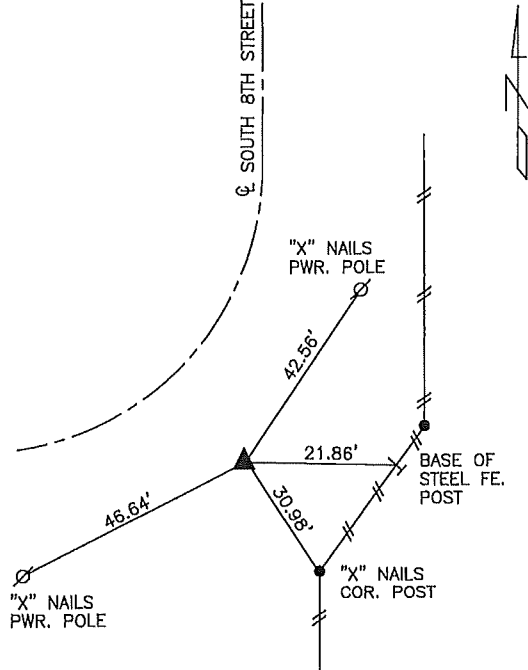
DISTANCES PLUMB CHAINED SE CORNER SECTION 15-83-39
