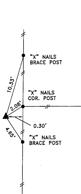
DISTANCES SLOPE CHAINED
