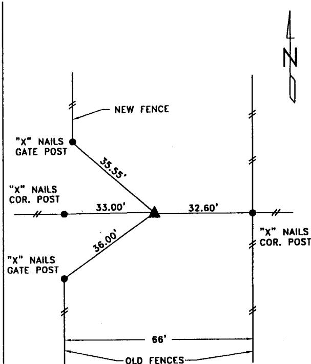
DISTANCES SLOPE CHAINED E1/4 CORNER OF SECTION 9-83-40
