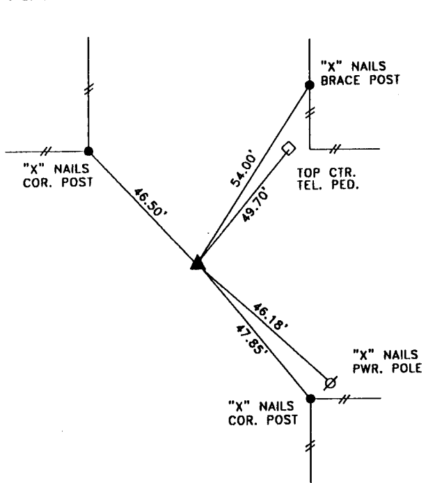
DISTANCES SLOPE CHAINED NE CORNER OF SECTION 9-83-40
