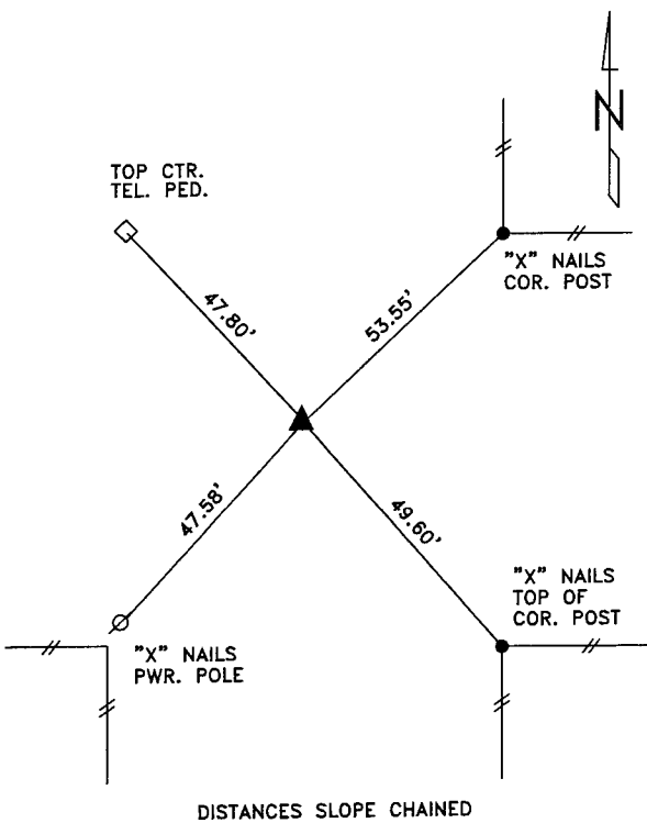
NW CORNER SECTION 32-85-38
