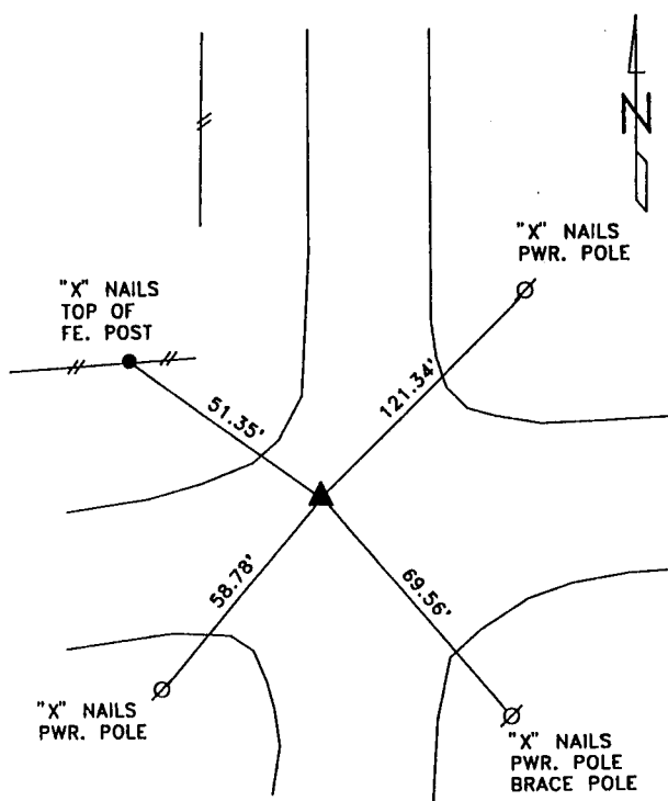
DISTANCES SLOPE CHAINED E1/4 CORNER SECTION 31-82-40
