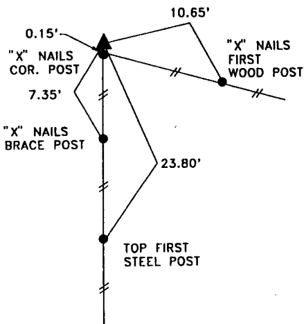
DISTANCES SLOPE CHAINED NE CORNER SECTION 31-82-40
