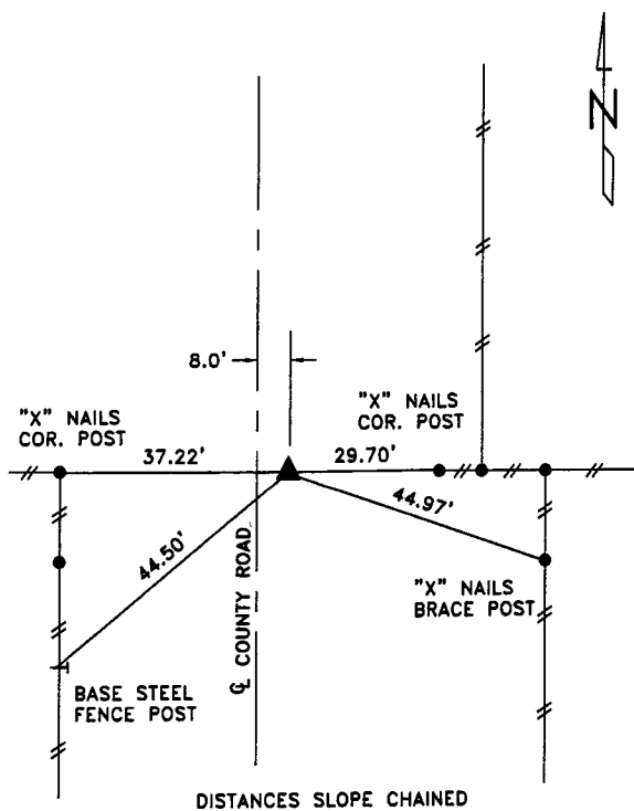
W1/4 CORNER SECTION 28-83-41
